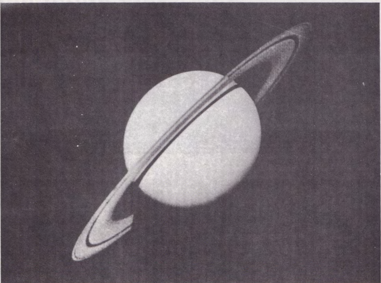
SATURN
